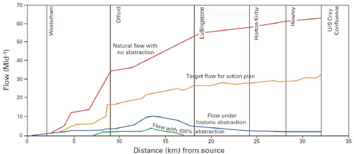
The figure illustrates the scheme [Darent Action Plan] by a comparison of actual and target flow accretion profiles for August, the former being based on 1976 and 1989/92 observations and, therefore, representing a late summer drought condition. (British Geological Society, 2008)
