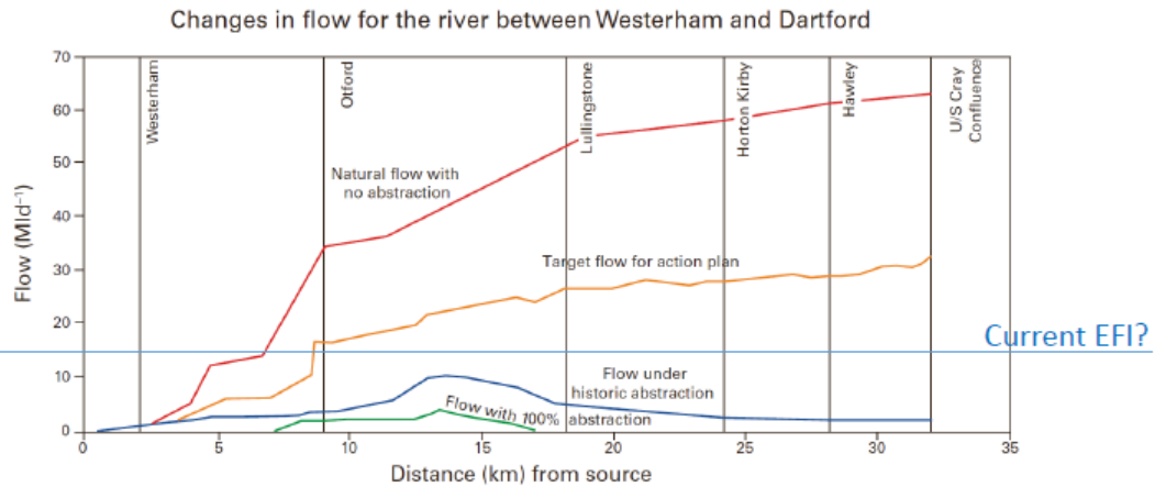
The figure illustrates the scheme by a comparison of actual and target flow accretion profiles for August, the former being based on 1976 and 1989/92 observations and, therefore, representing a late summer drought condition. (British Geological Society, 2008)
